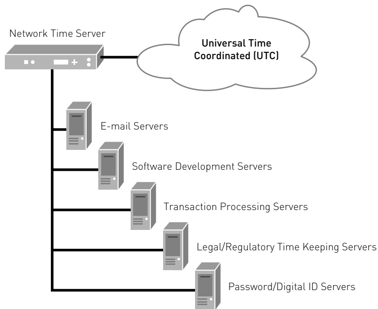
FIG.2 Typical applications needing network synchronization
