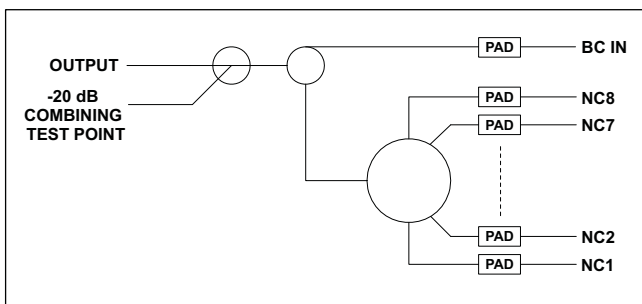
Functional Schematic
